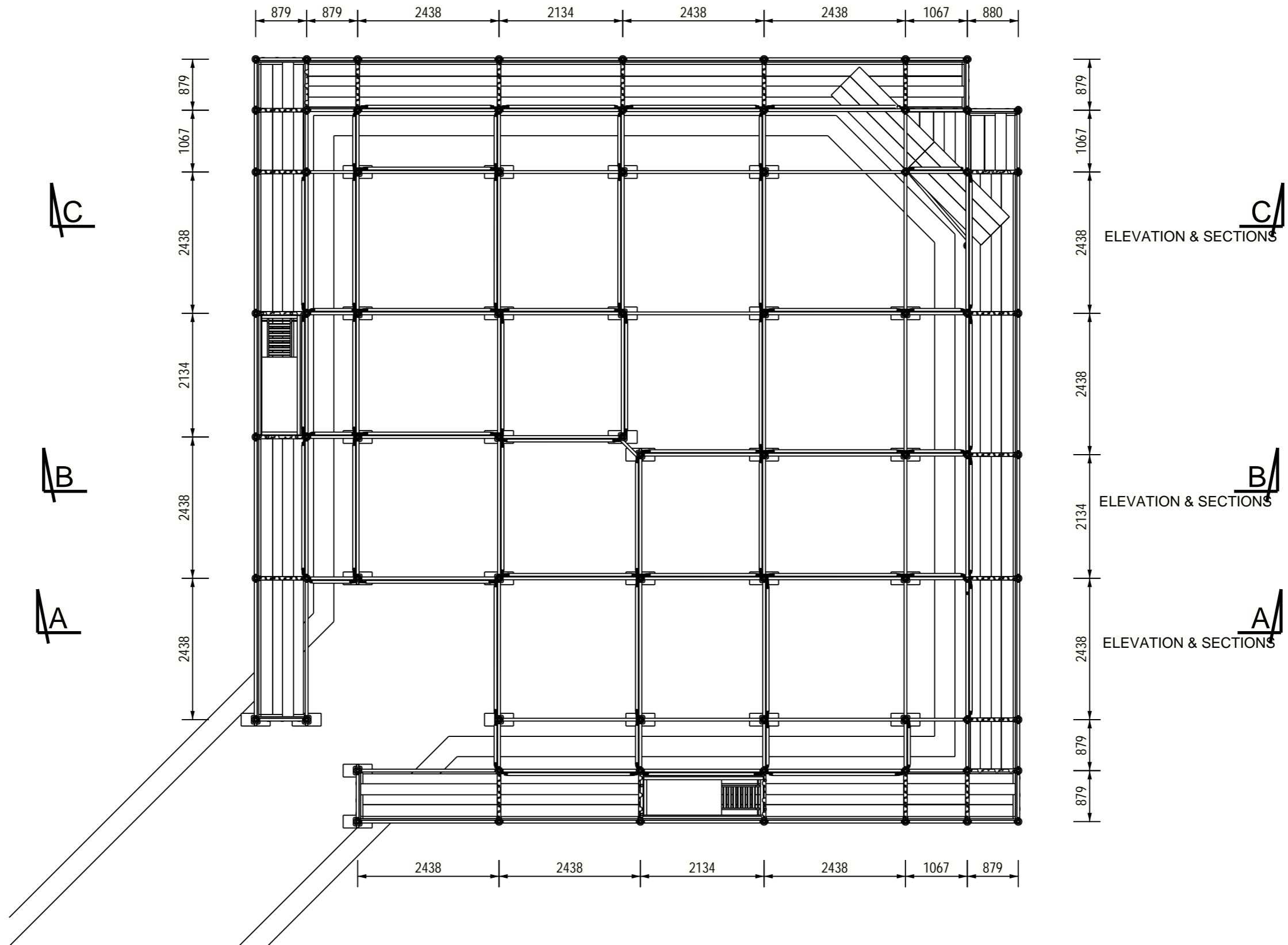
PLAN @ 1:75
