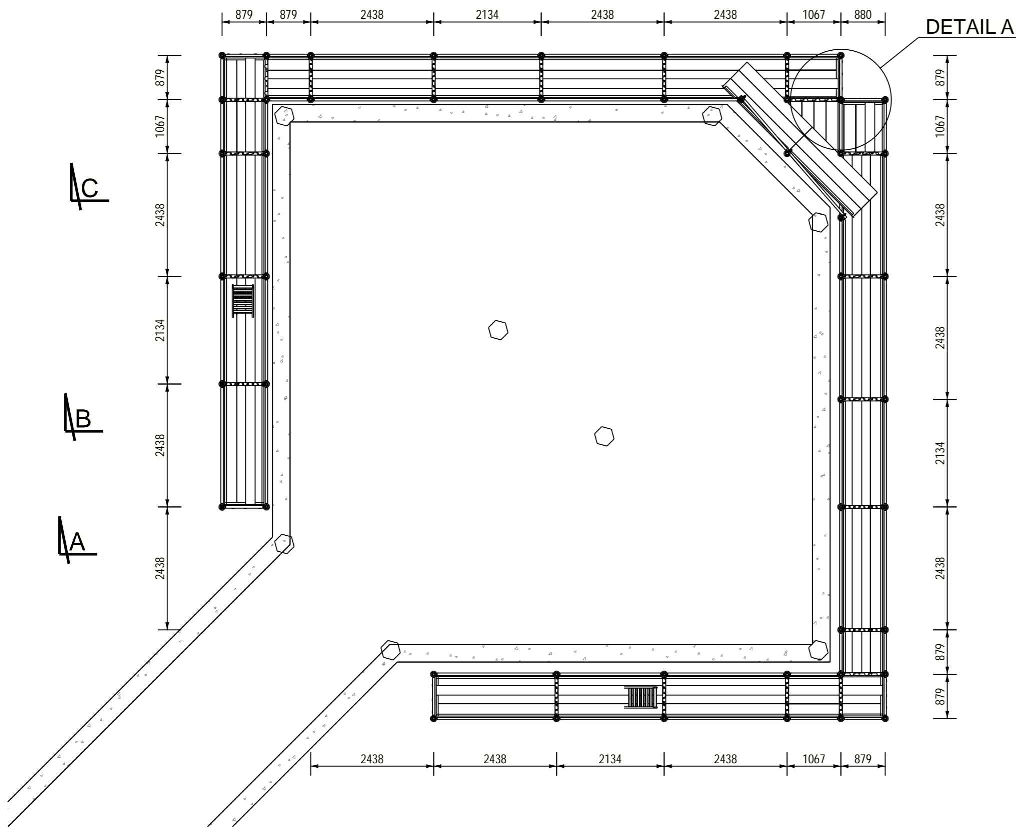
PLAN @ 1:75
