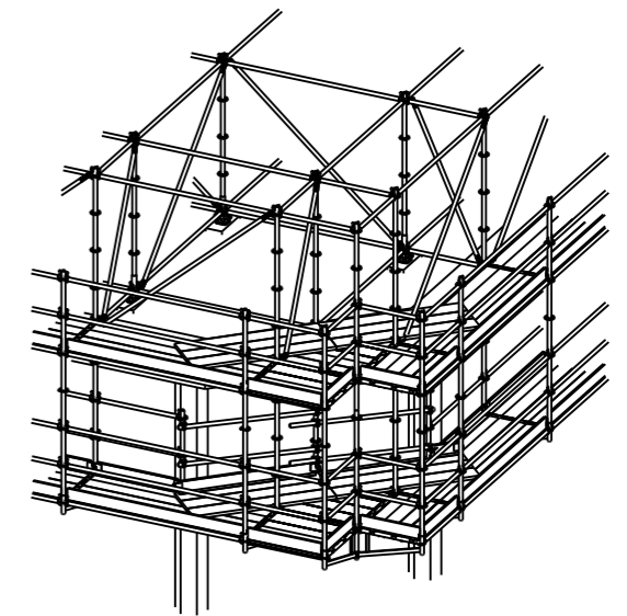
DETAIL A @ 1:100
