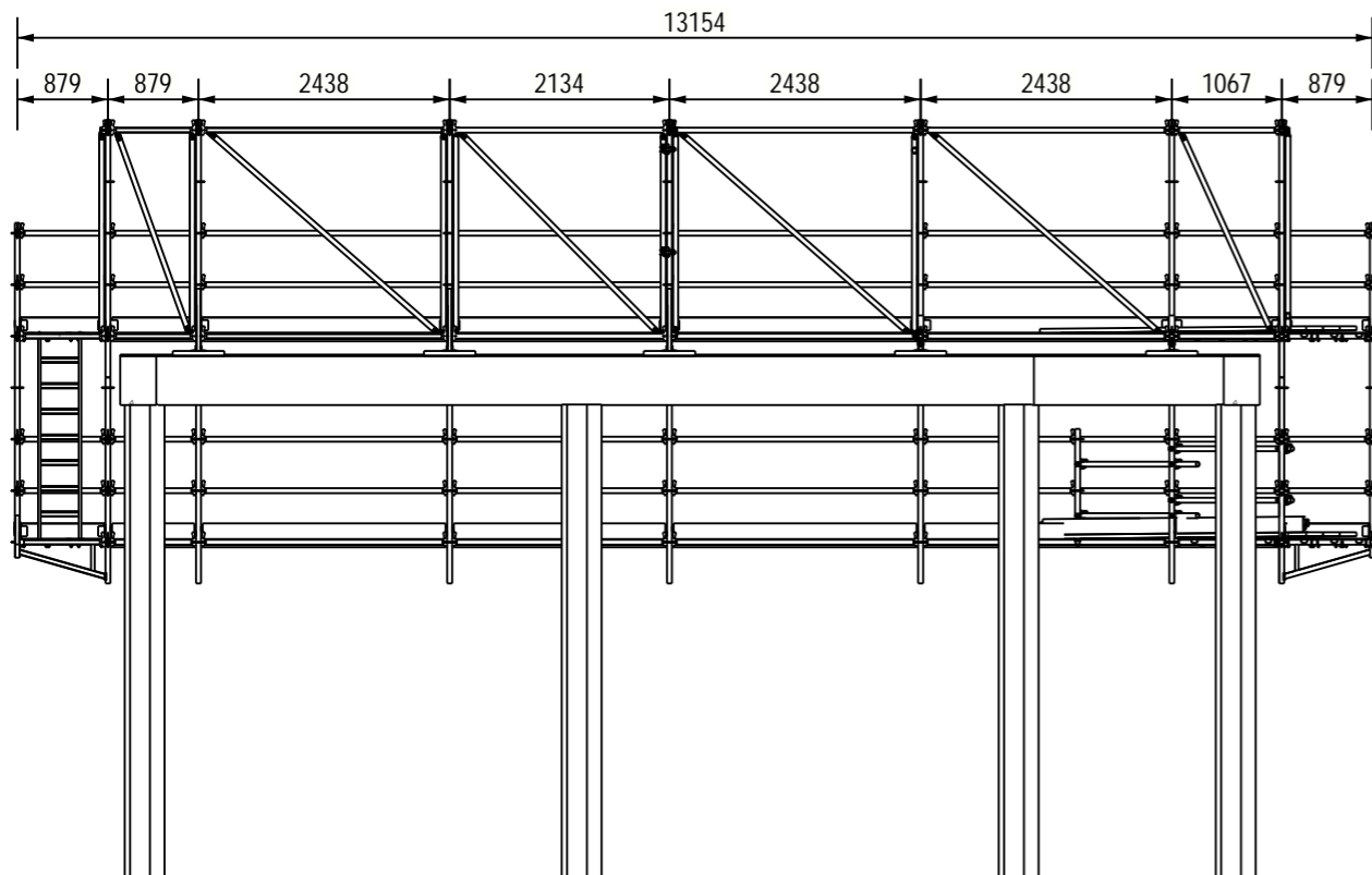
SECTIONS B - B 1:80 PLAN VIEW UPPER
