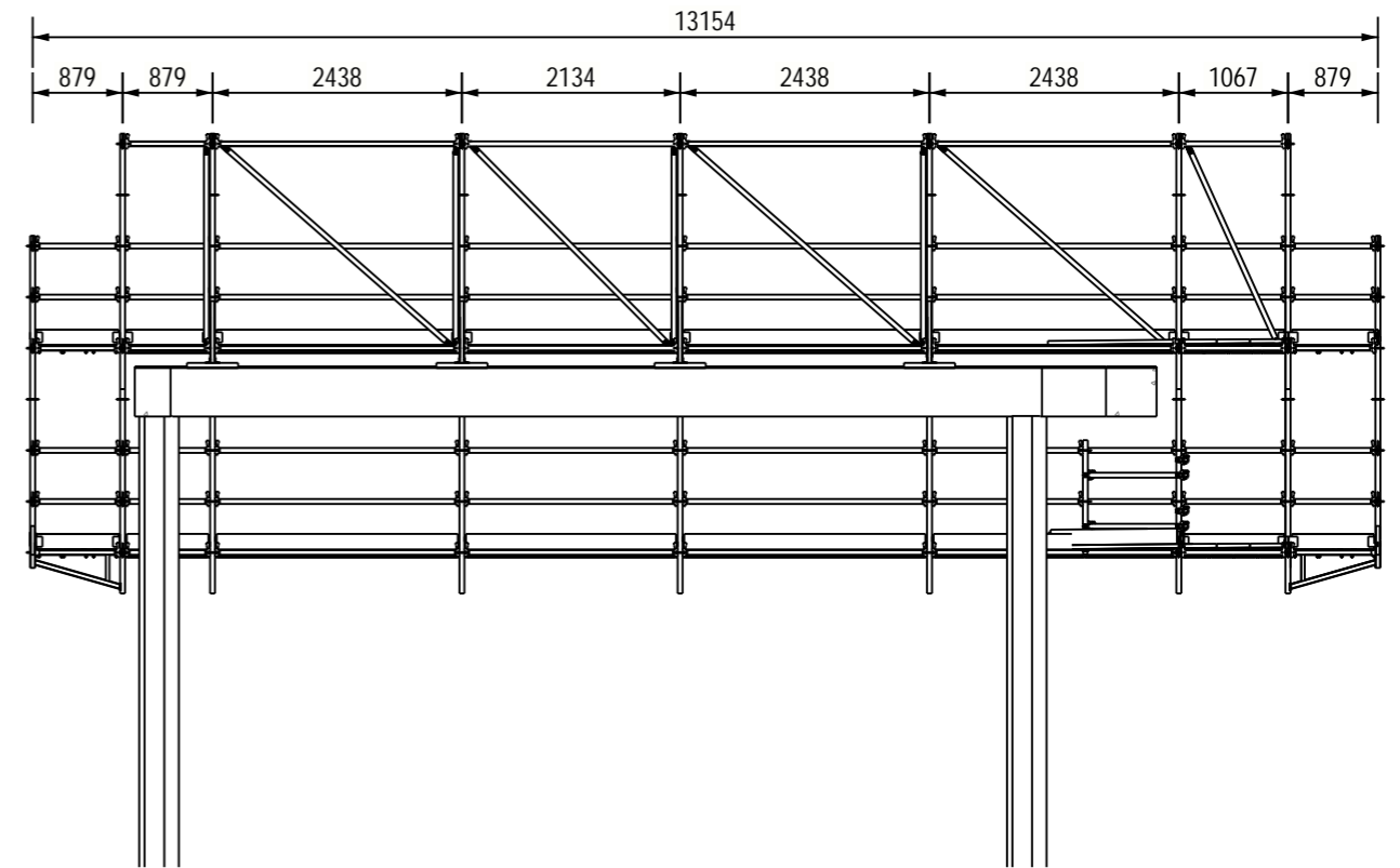
SECTIONS C - C 1:80 PLAN VIEW UPPER
