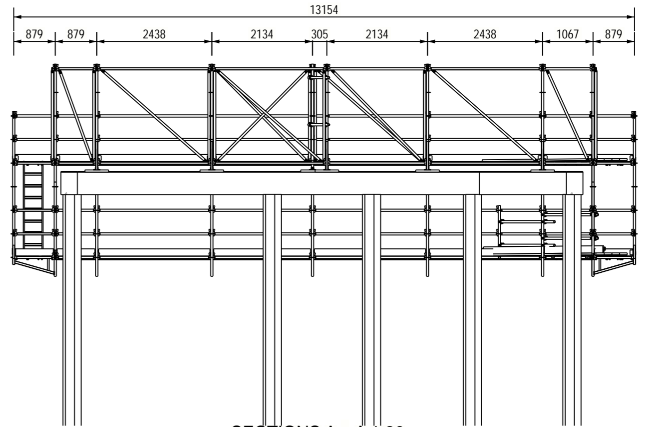
SECTIONS A - A 1:80 PLAN VIEW UPPER
